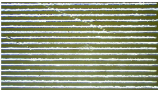
Fig. 7. Micrograph of bright surface on a solder coated Cu-FR4 interdigitated electrode with silicone encapsulation following aging. Imaged at 6.4B magnification.
