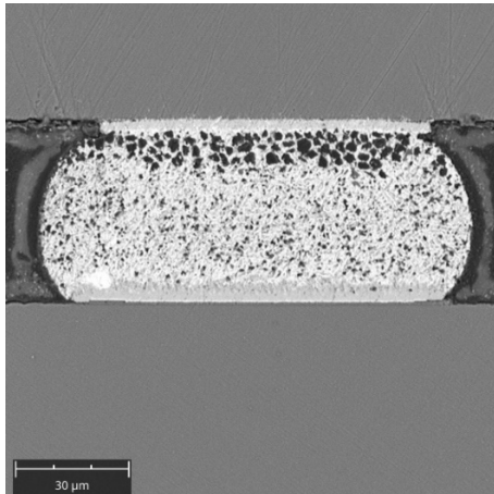
Figure 5: SEM micrograph depicting the cross-sectioned indium micro bump achieved through manual polishing.
