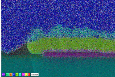
Figure 13: EDS analysis at crack interface
