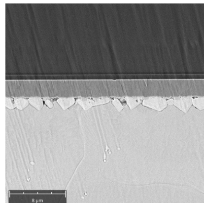
Figure 12: Identification of a crack at the top interface following the extended cryo-milling procedure.
