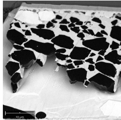
Figure 10: Tilted SEM image illustrating the presence of trapped particles within the soft texture of the indium bump.
