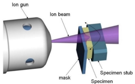
Figure 3: Ar Blade Cross-section Mode [5].
