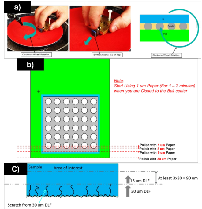
Figure 4: Guideline for mechanical polishing. a) polishing direction on a clockwise rotating wheel, b) guideline distance for switching from coarse to fine DLF as approaching toward indium bumps, c) schematic of the scratch-removing process from coarse to fine polish.
