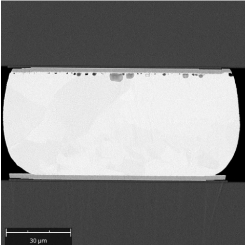
Figure 8: SEM image illustrating a clean and smooth surface of the indium bump cross-section achieved through Ar milling at -70^{\circ}\text{C} .
