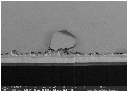
Figure 15: High-magnification SEM micrograph highlighting the presence of a crack at the indium/intermetallic interface.
