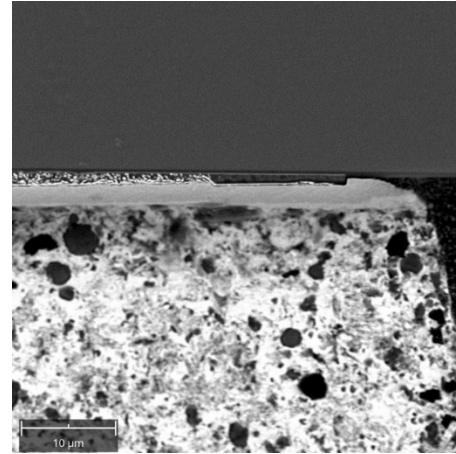
Figure 6: SEM micrograph illustrating the cross-sectioned indium micro bump that has been cleaned using the flat Ar milling procedure.
