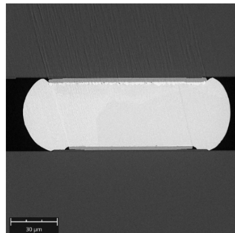
Figure 11: The extended Ar milling process notably enhances the quality of the cross-sectioned indium bump.
