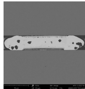
Figure 7: SEM image showcasing the Ar mill cross-section microstructure of the indium micro bump at room temperature.
