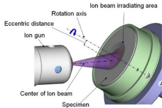
Figure 2: Ar Blade Flat Milling Mode [5]
