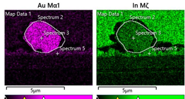
Figure 16: EDS mapping confirming the formation of a crack at the indium/intermetallic interface.
