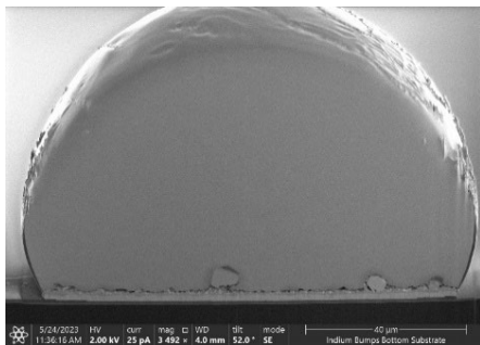
Figure 14: SEM image displaying the cross-section of the indium micro bump obtained through the PFIB technique.
