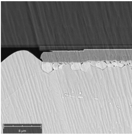
Figure 9: SEM image depicting a crack observed at the top interface.
