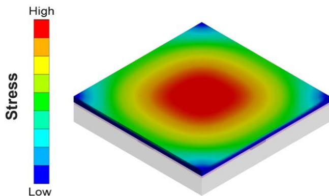
Figure 4: Filter glass deformation at elevated temperature in FEM simulation
