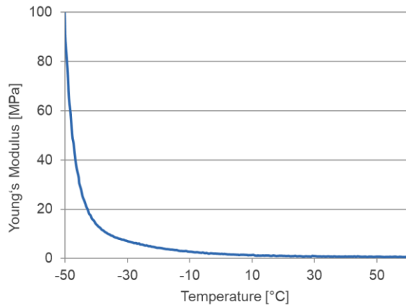
Figure 6: Young's Modulus over Temperature
