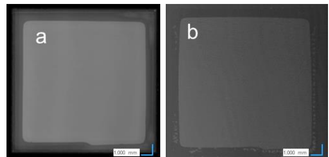
Figure 3: Bondline inspection by means of acoustic microscope on DELOs test vehicle
