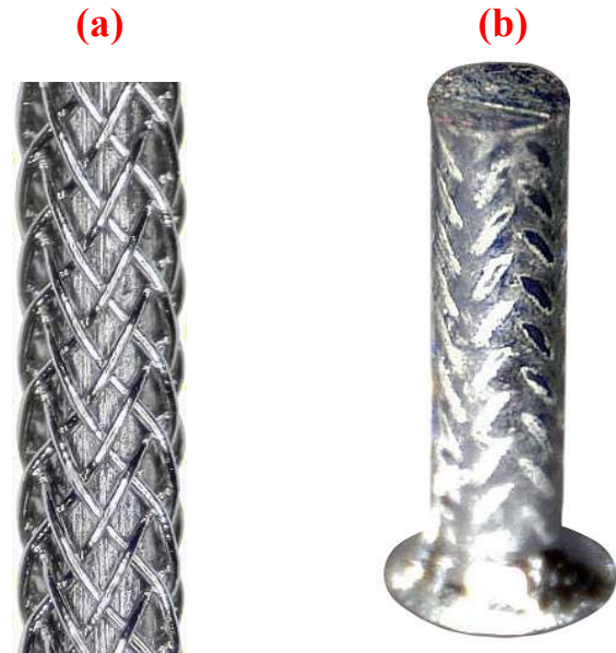
Fig. 1: (a) Copper Braided Solder Column shown prior to solder coating. (b) Braided Solder Column (after solder coating) with solder fillet mounted to a BGA pad.
