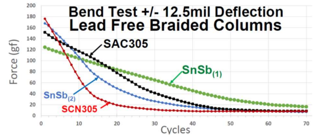
Fig. 7: Lead Free Columns subjected to Accelerated Bend Test +/-12.5mils Deflection. Best performance was observed with SnSb(1). Column diameter 0.50mm (20mil). Length 2.2mm (87mil). Braided BeCu wire diameter 25μm (1.0mil)
