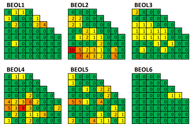
Fig. 3. Data maps of the upper right quadrant of each of the six BEOL test wafers summarizing the number of dielectric cracks manually detected by optical microscopy within each 5 mm x 5 mm die area following bond pad etching. The lower left box of each map corresponds to Die (09,09) whose lower left corner corresponds to the wafer center.
