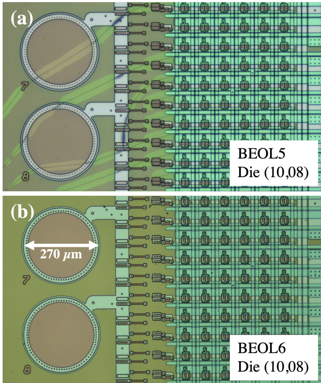
Fig. 2. Optical microscope photos of the identical regions of (a) BEOL5 and (b) BEOL6 recorded following deposition of the final 0.8 \mu\text{m} \text{SiO}_2 layer. This region of the BEOL5 wafer exhibited abundant dielectric layer cracks while no dielectric layer cracks are visible for same location on the BEOL6 wafer.
