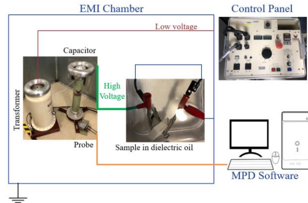
Figure 4: PDIV Test Setup
