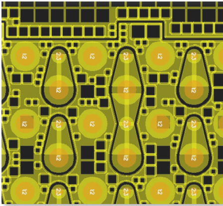
Figure 3. Density Control
