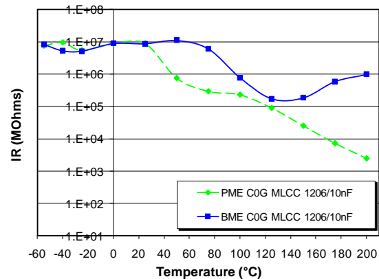
Figure 2. Dependence of IR on temperature with 25V DC bias for PME and BME COG MLCC.
