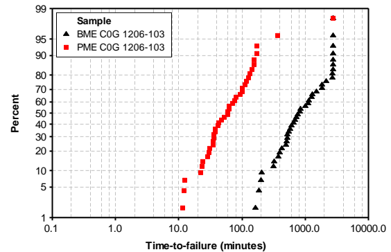
Figure 1. HALT for PME and BME COG 1206/10nF MLCCs. (HALT at 175^\circ\text{C} and 400V.)
