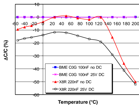
Figure 3. \Delta C/C variation with temperature and DC bias.
