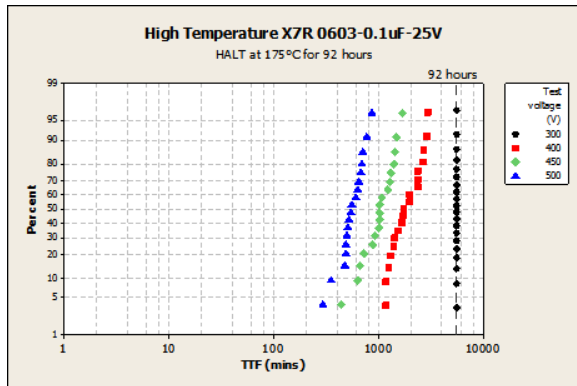
Figure 10. HALT testing time-to-failure (TTF, minutes) plot for Modified-X7R 0603-0.1µF capacitors (rated at 25V) at 175°C for 92 hours
