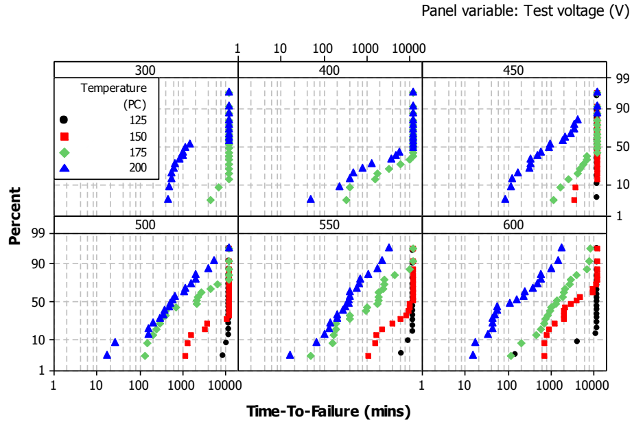
Figure 7(a). HALT distributions at various test conditions for 0805- 2200 pF 50V.
