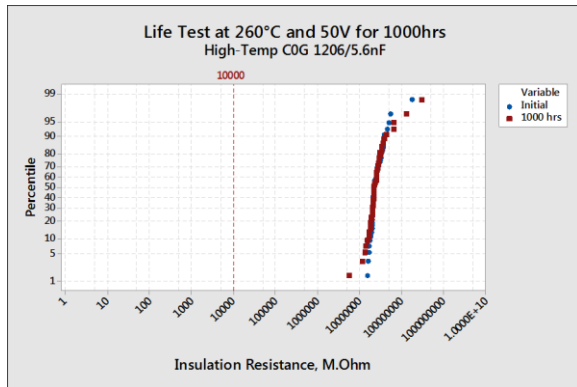
Figure 8. Insulation resistance (IR) plot after Life Test of High Temperature COG 1206-5.6nF capacitors at 50V and 260°C for 1000 hours.
