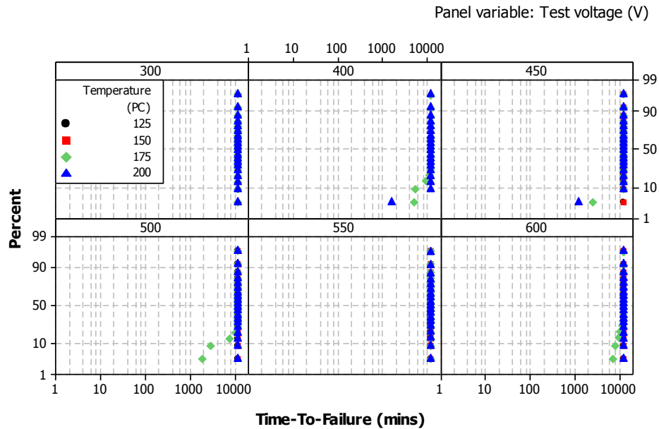
Figure 7(b). HALT distributions at various test conditions for 0603-470 pF-50V.
