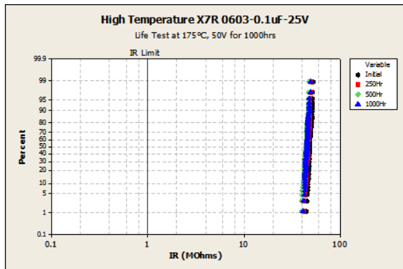
Figure 11. Insulation resistance (IR) plot after Life Test of Modified-X7R 0603-0.1µF capacitors (rated 25V) at 50V and 175°C for 1000hrs hours
