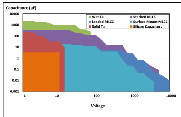
Fig. 1. Capacitance vs. Voltage ranges of different capacitor types rated at 200°C.
