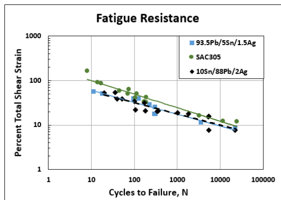
Fig. 16. Fatigue Resistance of Different Solders
