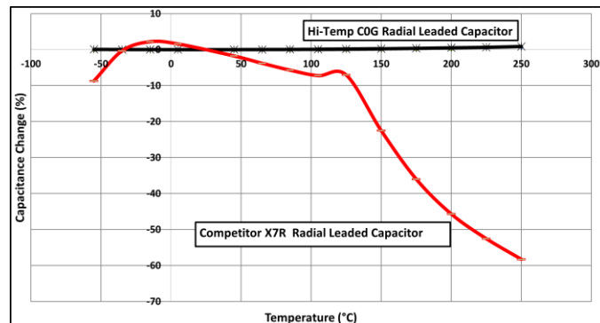
Fig. 2. Capacitance Change with Temperature for radial leaded HT C0G (0.22 \mu\text{F} ) vs. competitor X7R (1.2 \mu\text{F} ) both rated 100V.
