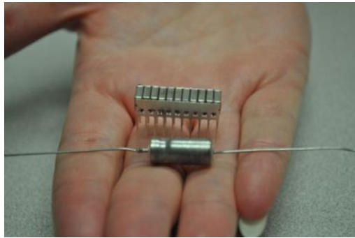
Fig. 4. Size Comparison of Wet Ta to MLCC Stack made with HT C0G.
