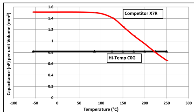
Fig. 3. Capacitance per Unit Volume for radial leaded HT C0G vs. competitor X7R.
