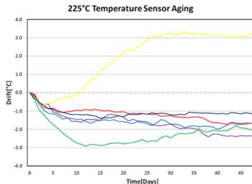
Figure 8 225°C Aging
