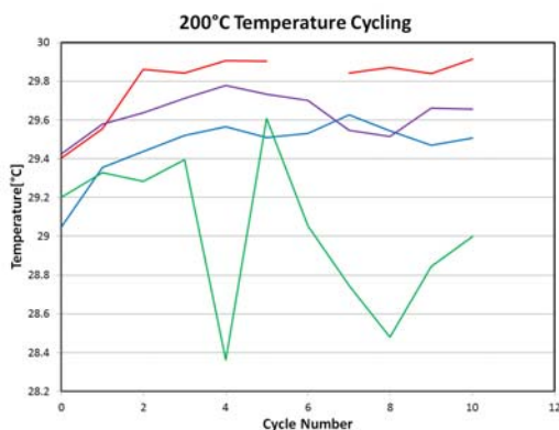
Figure 11 200°C Temperature Cycling
