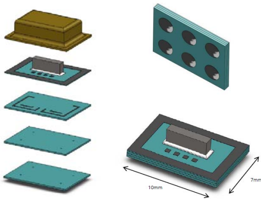
Figure 10: Packaging concept of aerosol contacted g-accelerometer in LTCC
