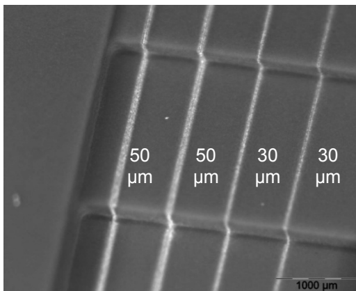
Figure 6: 3D printing on LTCC stairways (step height 220 μm, DP 951) with aerosol printed Ag micro ink.
