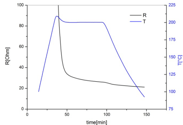
Figure 8: Sintering curve of the applied Ag nano ink (test structure embedded in LTCC DP 951).
