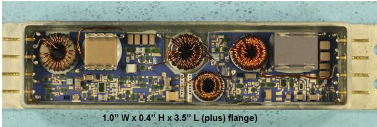
Fig (3) – Photo of Open Assembly of VHB Converter
