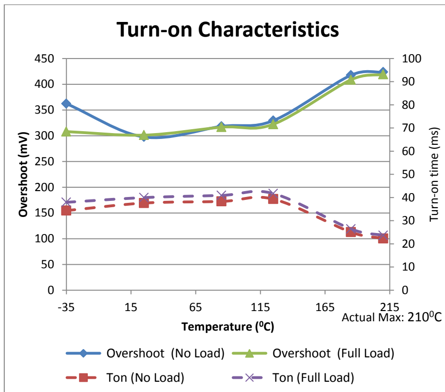
Fig. (18) Turn on characteristics with overshoot amplitude and time duration vs. Temperature.
