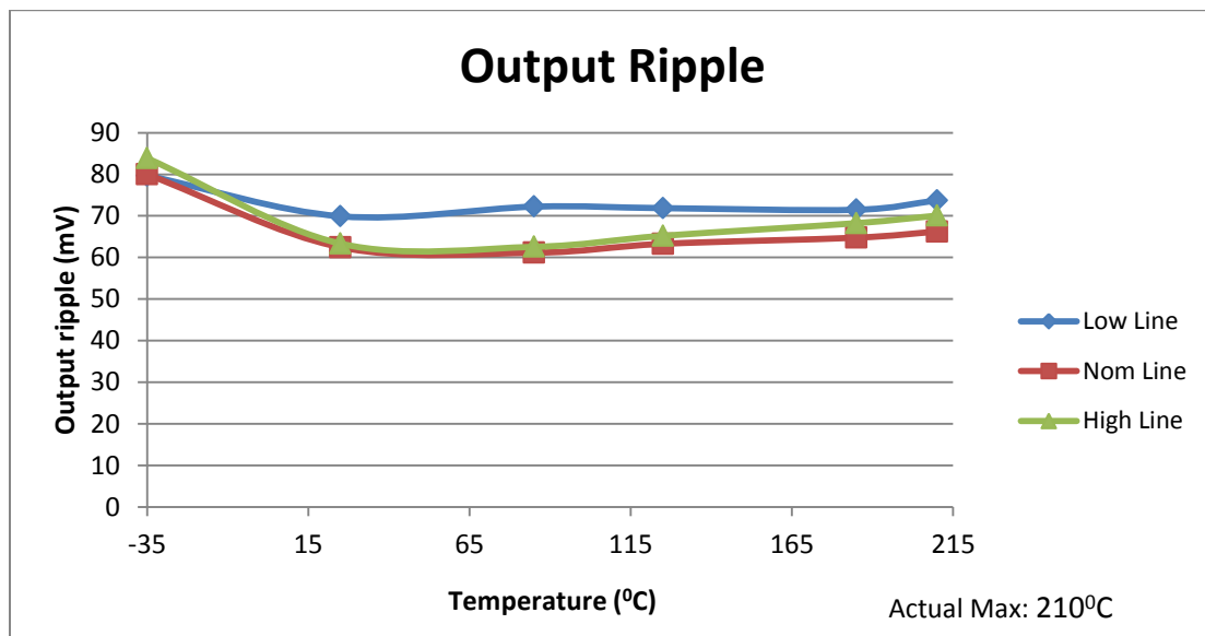
Fig. (16) Output ripple vs. temperature of VHB2805S at three line voltages
