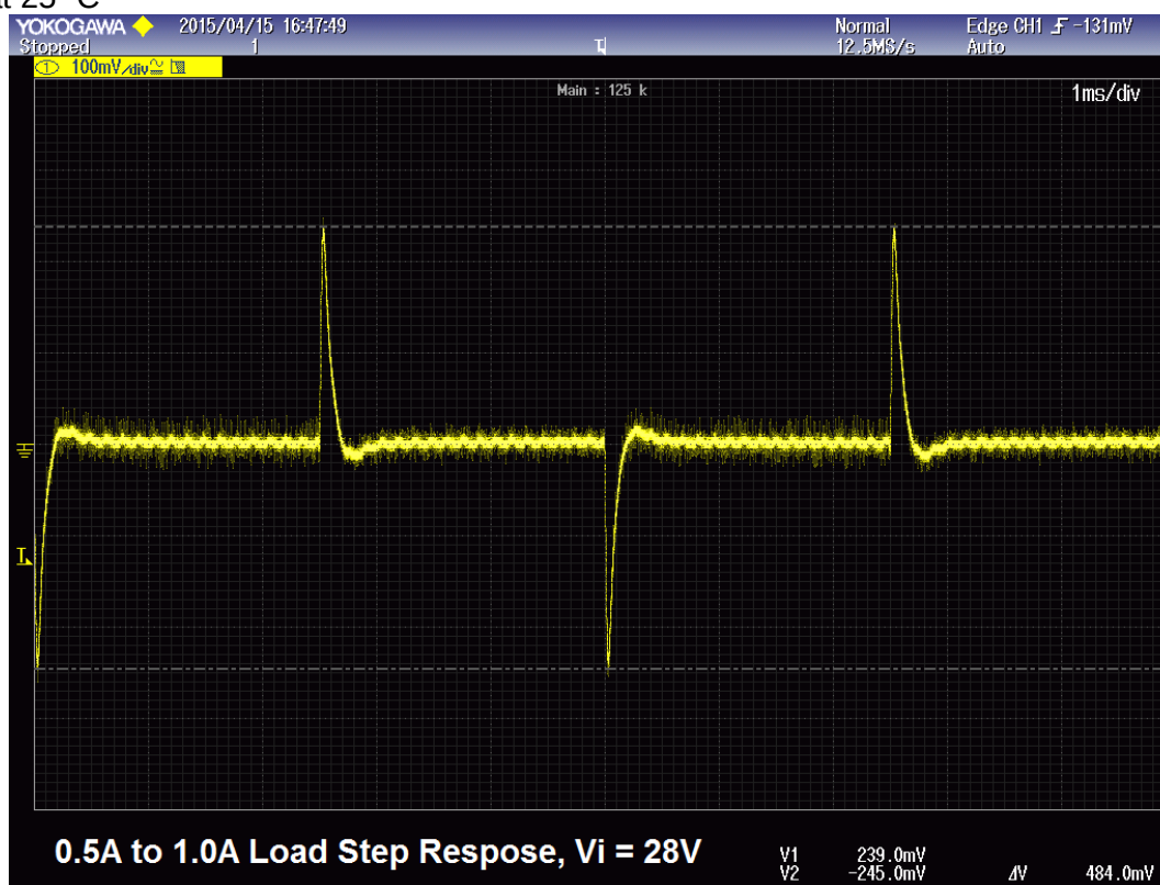
Fig. (11) Dynamic response of output voltage when load is switched from 50% to 100% with input=28VDC at 25 °C
