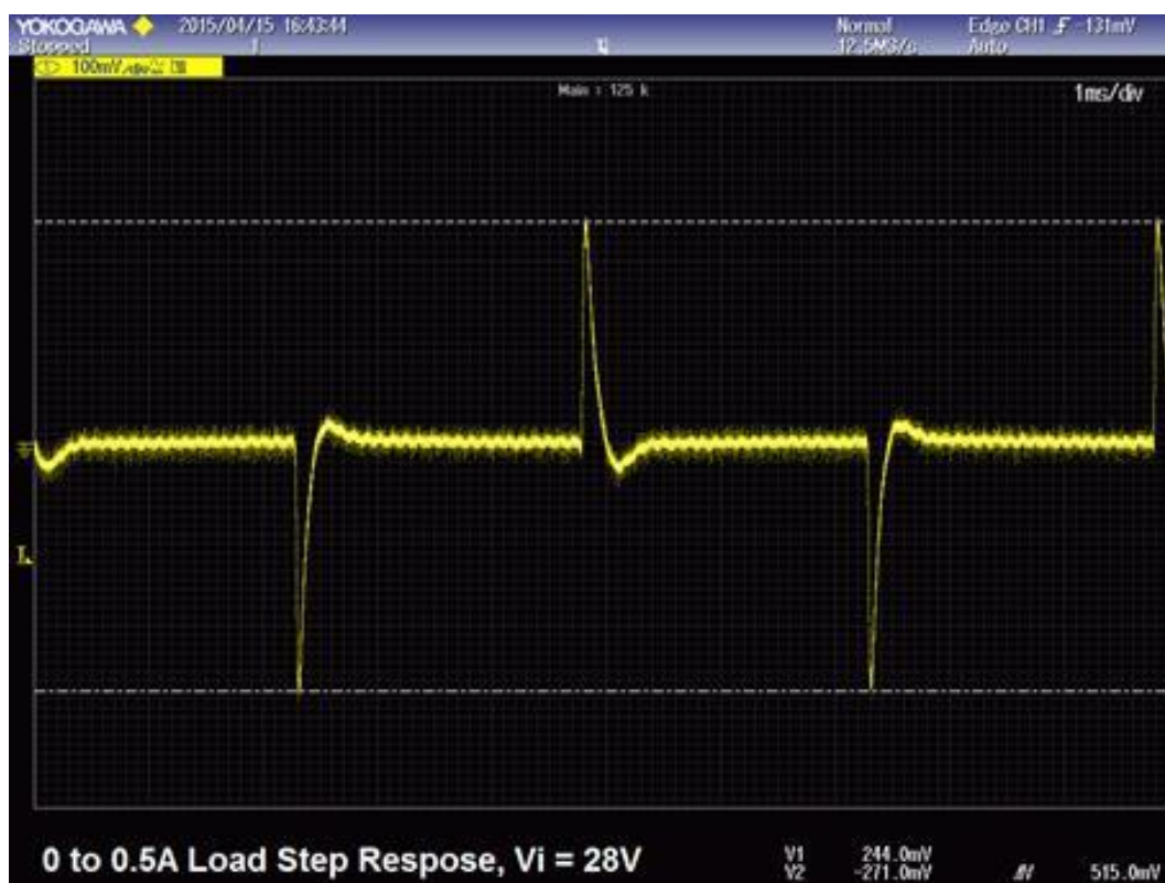
Fig. (10) Dynamic Response of output when input=28VC and output load is switched from 0.0 to 50% at 25 °C
