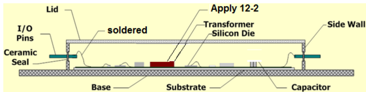
Fig. (4) Assembly, Design and Construction of Hybrid
