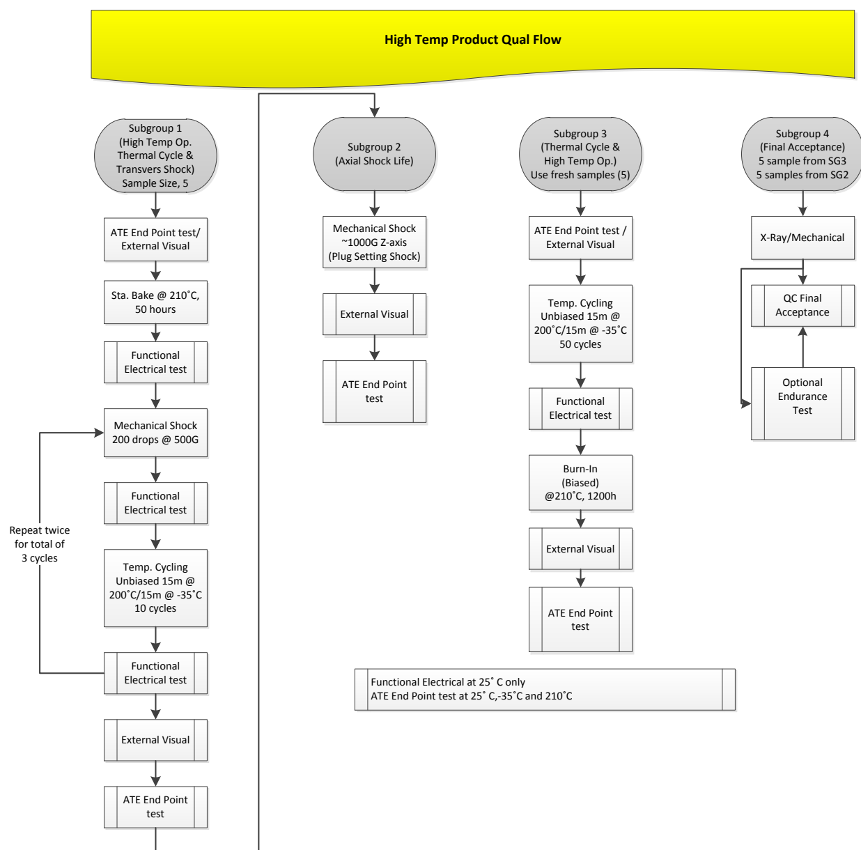
Fig. (20) High Temp product Qual Flow.
