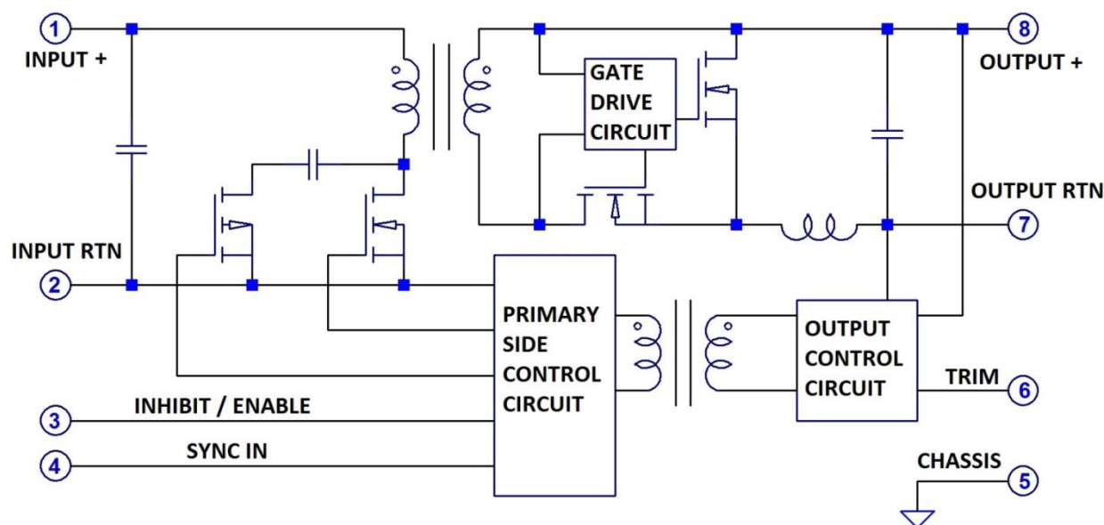
Fig (2) – Functional Block Diagram of VHB Converter
