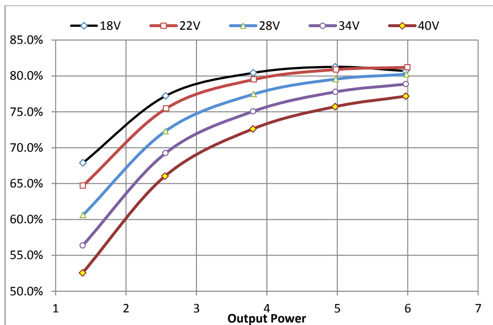
Fig. (6) VHB2805A % Efficiency vs. output power in watts at 215 °C
