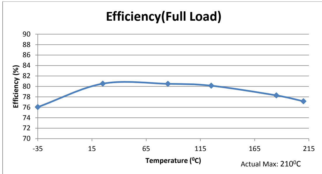
Fig. (15) Efficiency at full load vs. Temperature of VHB2805S
