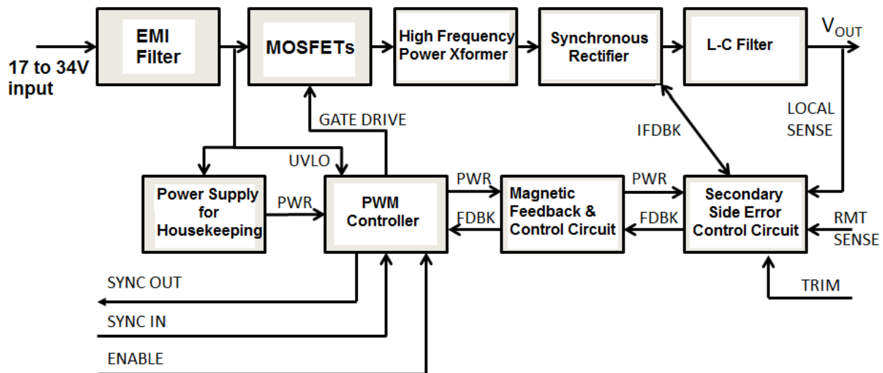
Fig. (1) Block Diagram showing Topology of VHB DC to DC Converters
