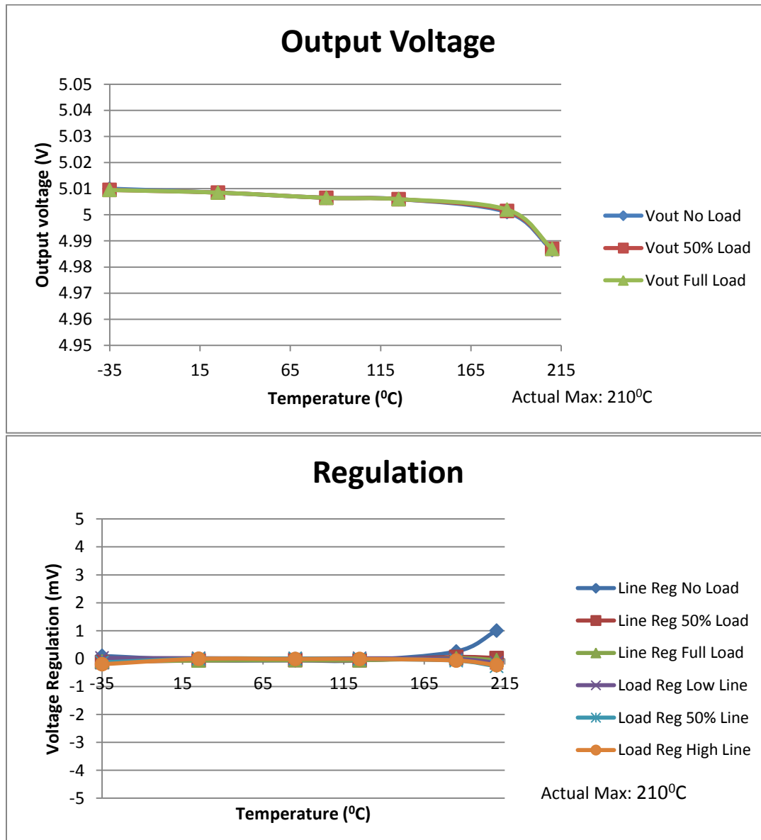
Fig. (14) Output Voltage and Regulation vs. Temperature of VHB2805S
