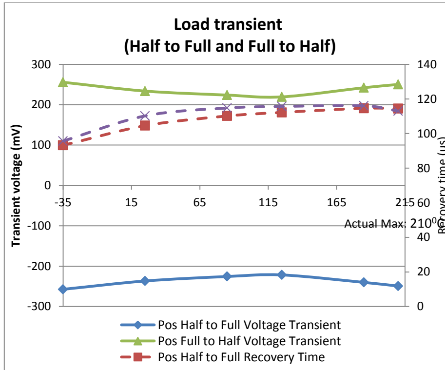
Fig. (17) Load transient response in amplitude and time for different changes in loads
