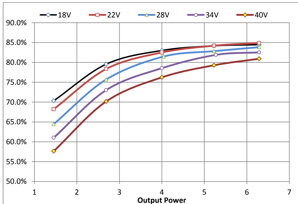
Fig. (5) VHB % Efficiency vs. output power in watts at 25 °C
