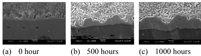
Fig. 7 IMC growth and morphology changes subject to thermal aging at 125^\circ\text{C} (ENIG)
