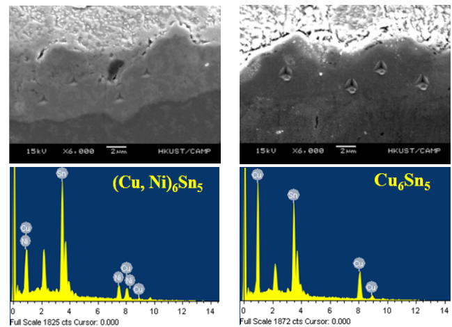
Fig. 8 SEM and EDX analysis of IMCs
