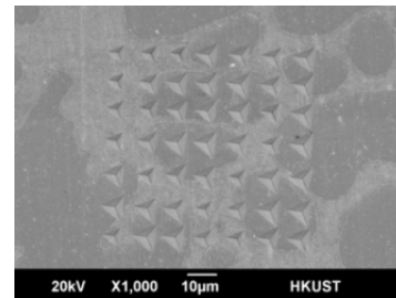
(a) Typical indentation marks on SAC lead-free solder joint
