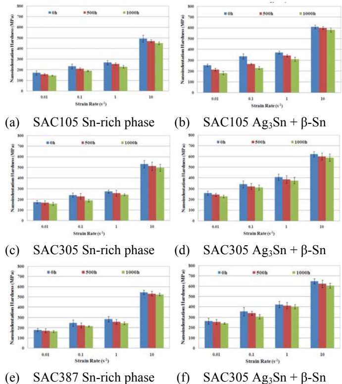
Fig. 5 Comparisons of nanoindentation hardness of the SAC lead-free solder joints
