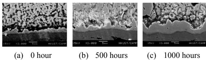
Fig. 6 IMC growth and morphology changes subject to thermal aging at 125^\circ\text{C} (OSP)
