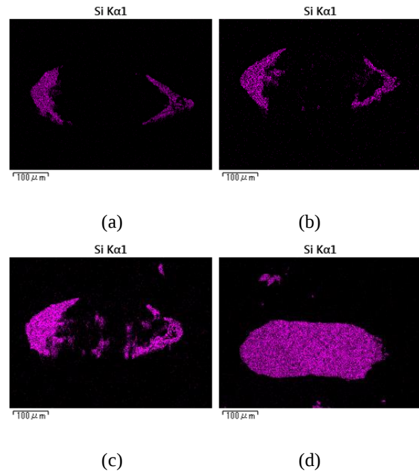
Fig. 4 Si mapping of pad surface after shear test (a) Before annealing (b) 200°C for 10 hrs (c) 200°C for 50 hrs (d) 300°C for 100 hrs
