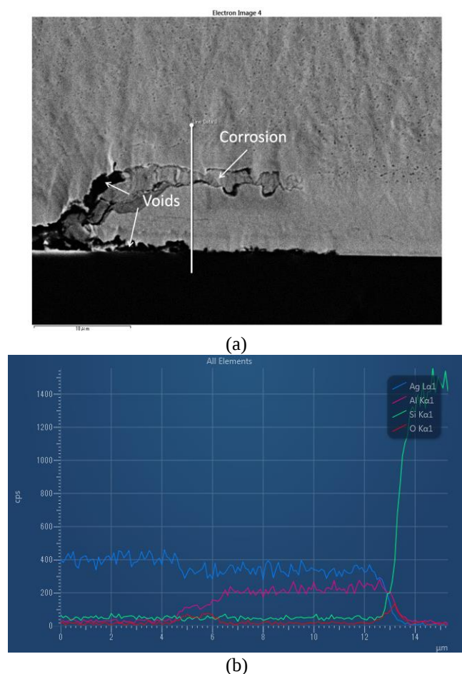
Fig. 8 Ag wedge bonding annealed in 300°C for 3 hrs with molded IC packages (a) SEM view (b) EDS line analysis
