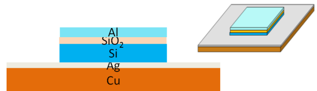
Fig 1. The structure of bonding pad
