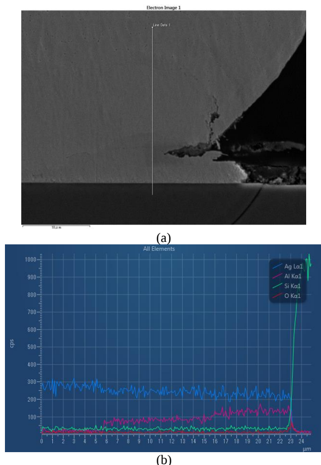
Fig. 5 Ag wedge bonding annealed at 300 °C for 50 hrs in air (a) SEM view (b) EDS line analysis
