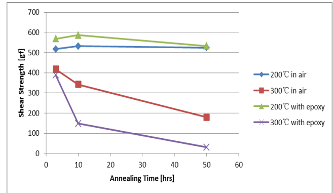
Fig. 3 Shear test of Ag wedge bonding
