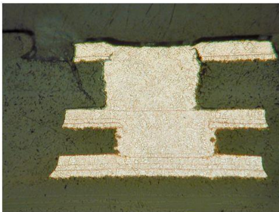
Figure 7: Copper filled microvia with corner crack. Source: Paul Reid [12]
