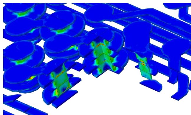
Figure 11: First principle stress ( \sigma_1 ) plot for a stacked via
