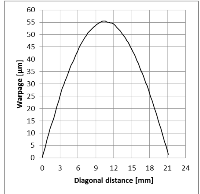
Figure 5: Predicted diagonal warpage
