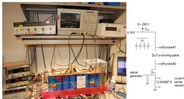
Figure 1. Experimental Set Up for Wire Fuse, and Schematic Diagram for the Circuit
