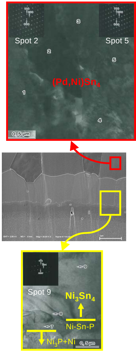
Fig.-8 TEM and FE-SEM observations on IMC with Sn-3.5Ag soldered to ENEPIG deposit after heat treatment applied at a temperature of 150°C for a period of 1,000 hours
