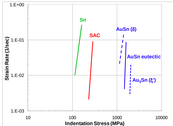
Figure 3: Creep strain rate versus indentation stress for solders and intermetallics, as measured by nanoindentation [35].
