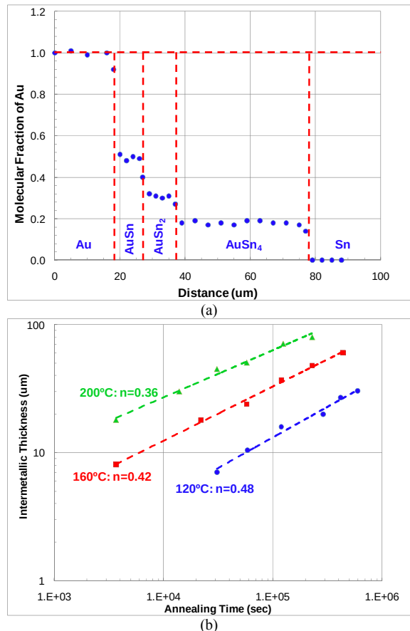
Figure 4: (a) Intermetallic formation in Au-Sn diffusion couple after 127 hrs at 160°C [39]; (b) total intermetallic thickness ( \text{AuSn}_4 + \text{AuSn}_2 + \text{AuSn} ) as a function of annealing time at different temperatures, with the associated time exponent in Equation 1 [31,39].
