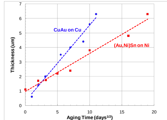
Figure 2: Consumption of barrier metallization by intermetallic versus time at 200°C for eutectic AuSn solder on Ni UBM and bare Cu [19,40].
