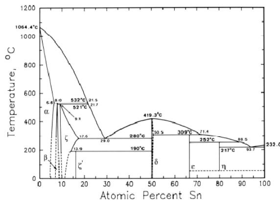
Figure 1: Au-Sn binary phase diagram (adapted from [1]).
