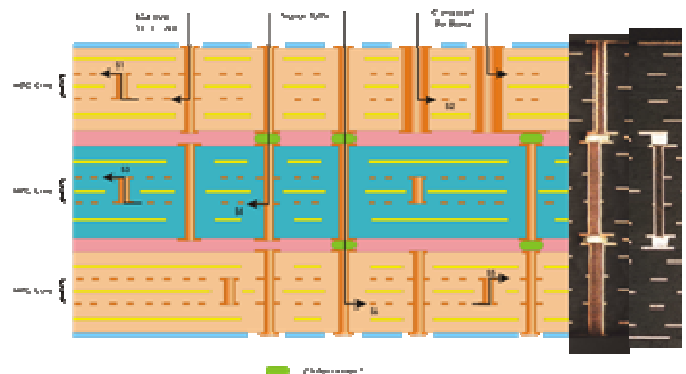
Figure 1 Z-interconnect cross-section
