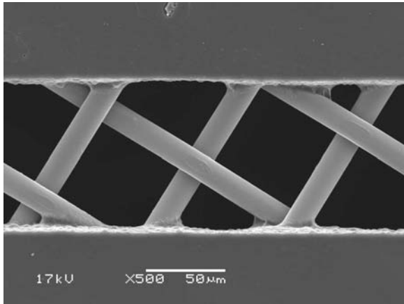
Figure 3. 360 mesh screen, 15μm wire diameter, 100μm finger line opening, 27μm EOM. Open area is 60.0%. SEM photo is directly over finger line opening, 500x.
