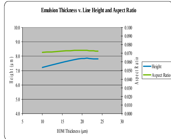
Figure 4. Emulsion Thickness v. Line Height and Aspect Ratio. 360 mesh screen, 15μm wire diameter.
