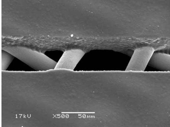
Figure 5. 280 mesh, 25µm wire diameter, 60µm finger line opening, 24µm EOM. SEM photo was taken at 30° from the top view, 500x.
