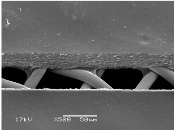
Figure 6. 360 mesh, 15µm wire diameter, 60µm finger line opening, 27µm EOM. SEM photo was taken at 30° from the top view, 500x.
