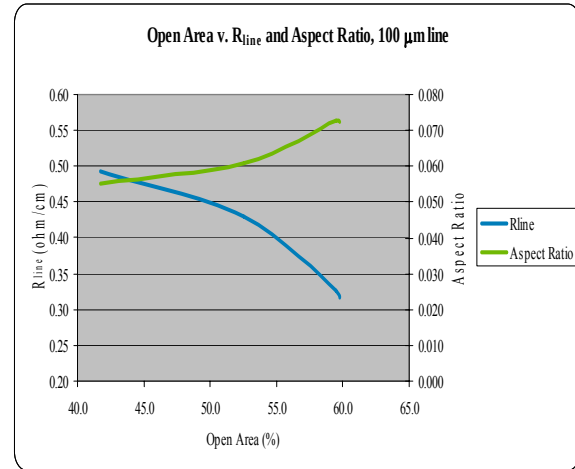
Figure 1. Open Area % v. R_{\text{line}} and Aspect Ratio. Averaged data from the 100 \mu\text{m} finger line openings.
