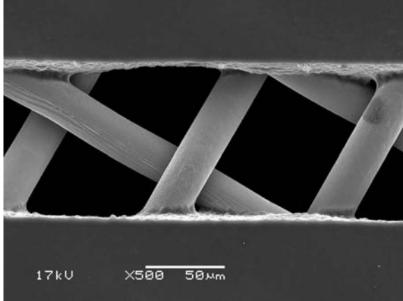
Figure 2. 280 mesh, 25μm wire diameter, 100μm finger line opening, 24μm EOM. Open area is 52.5%. SEM photo is directly over finger line opening, 500x.
