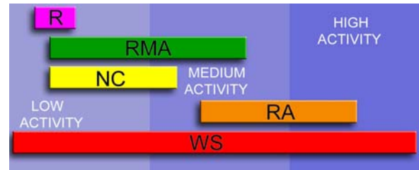
Figure 1: Flux Comparison Chart
