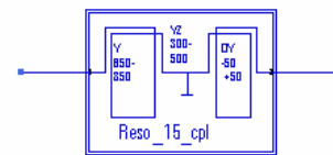
Figure 8 A complex LTCC mechanical object, comprising a pair of coupled resonators.
