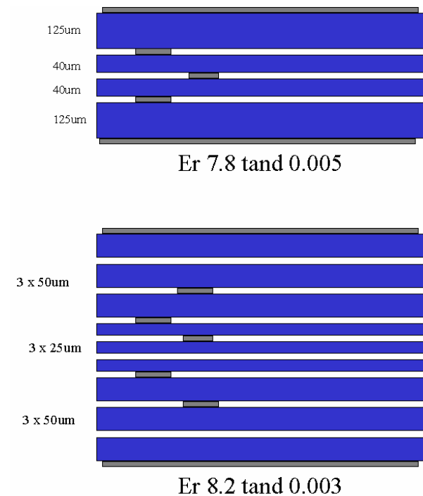
Figure 10 A comparison of 2 different LTCC stacks for the same filter.
