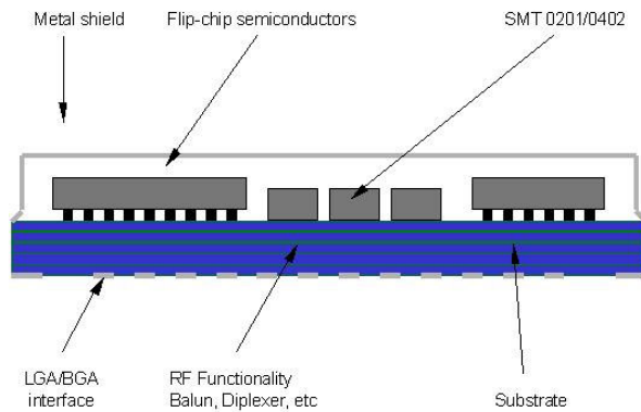
Figure 1 A typical RF SiP showing active components and buried functionality.
