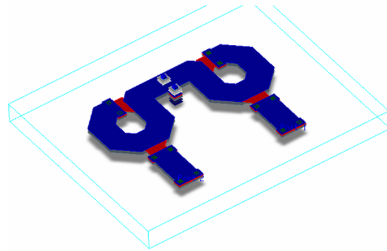
Figure 8 A complex LTCC mechanical object, comprising a pair of coupled resonators.
