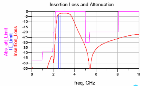
Figure 13 Electrical Performance
