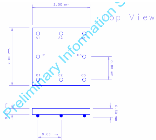
Figure 12 IPD filter layout.
