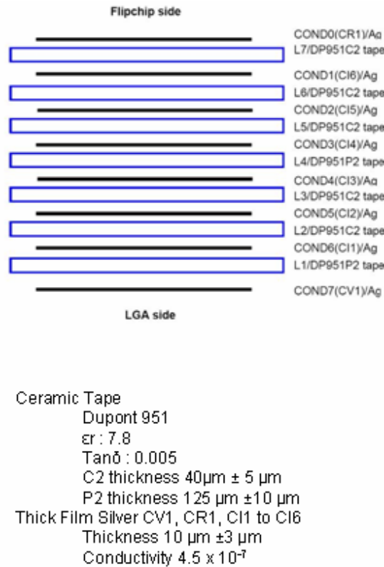
Figure 4 A typical LTCC technology file.
