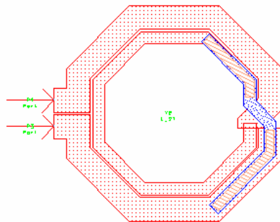
Figure 7 A typical IPD mechanical object, showing the parametric object with 2 distinct sets of parameters.
