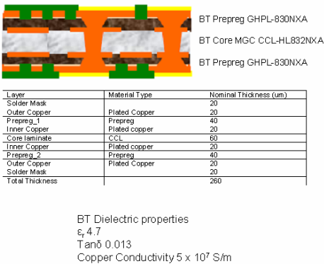
Figure 6 A typical laminate technology file.
