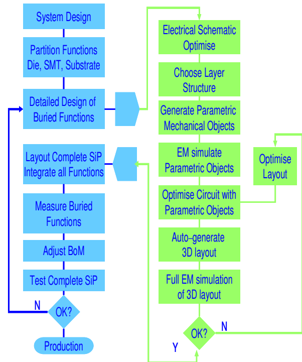
Figure 2 Flow diagram of Insight SiP's design methodology.
