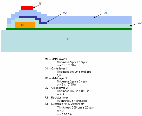
Figure 5 A typical IPD technology file.
