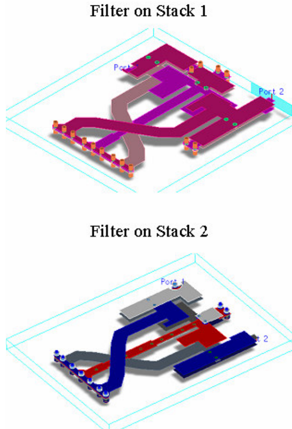
Figure 11 A comparison of full layout of filters, designed to have the same performance on 2 different LTCC stacks.
