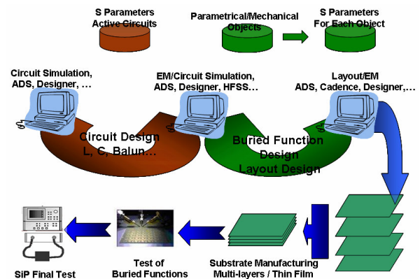
Figure 3 Design flow and tool usage for buried function design from schematic to layout.
