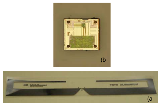
Figure 2: (a) Etched aluminum UHF antenna; (b) impinging gen-2 die.
