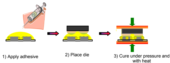
Figure 1: Schematic drawing of ACP assembly.
