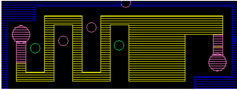
Figure 6 – Embedded Serpentine 10,000 Ohm Resistor with Vias in Legs – 1.0 mm x 3.3 mm
