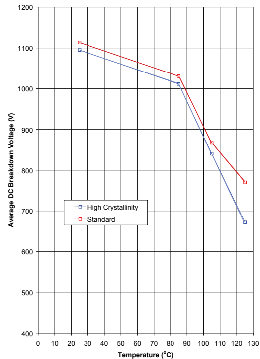
Figure 1 - Breakdown strength data with respect to temperature for small capacitors and two types of polypropylene film[7]
