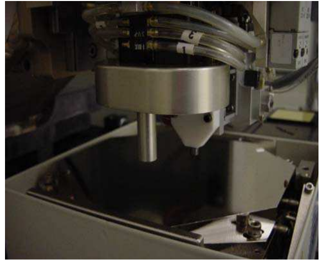
Palomar Technologies Model 6500 WSP features a heated wafer stage and heated bonding tool
