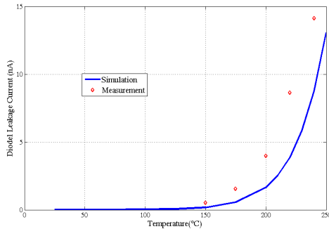
Fig. 8. Diode leakage current vs. temperature.
