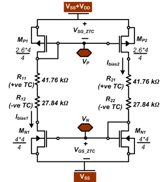
Fig. 4. Schematic of the temperature independent current bias network.
