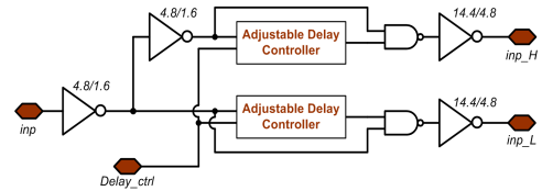
Fig. 3. Temperature independent dead-time controller circuit.
