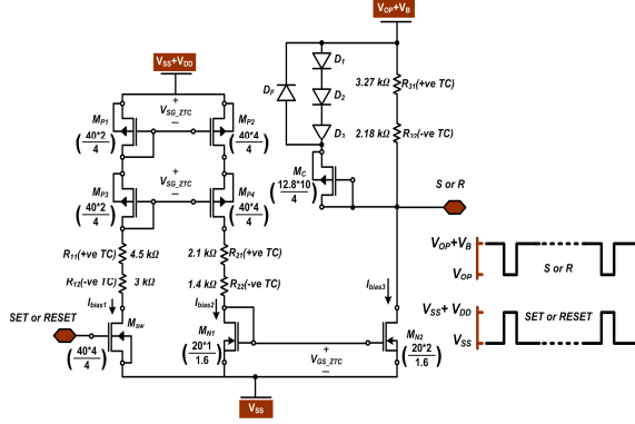
Fig. 7. Schematic of the temperature independent level shifter circuit.
