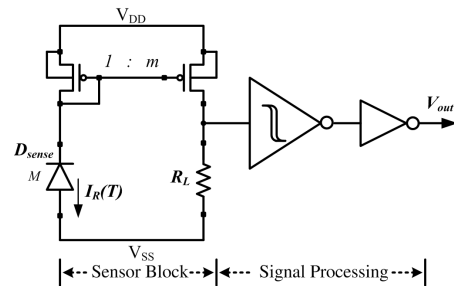
Fig. 9. Schematic of the proposed low-power on-chip temperature sensor circuit.
