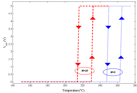
Fig. 12. Temperature sensor circuit's output with the increase and decrease of die temperature.
