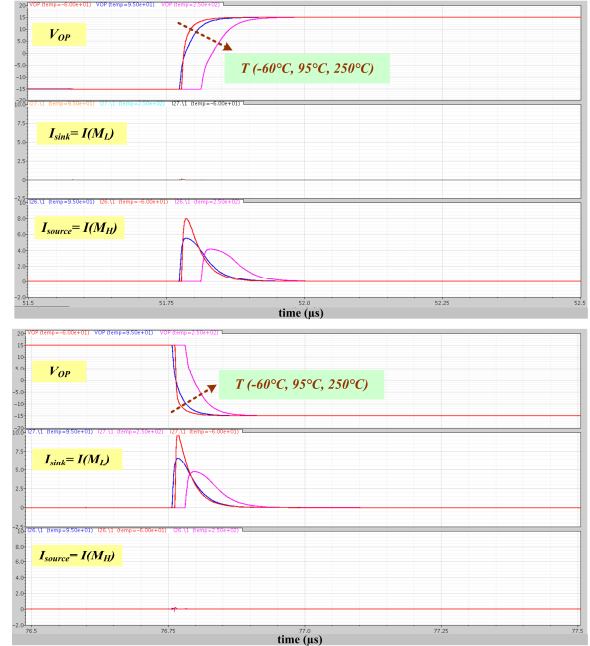
Fig. 11. Simulation results of the proposed high-temperature gate driver circuit at different temperatures (Red: -60^{\circ}\text{C} , Blue: 95^{\circ}\text{C} , and Pink: 250^{\circ}\text{C} ).
