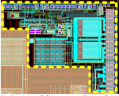
Fig. 10. Layout of the proposed gate driver and temperature sensor circuit.
