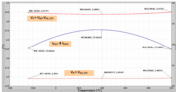
Fig. 5. DC simulation results of the temperature independent bias network.
