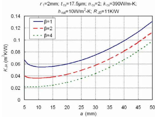
Figure 6. Effect of a on K_{JA} for different \beta
