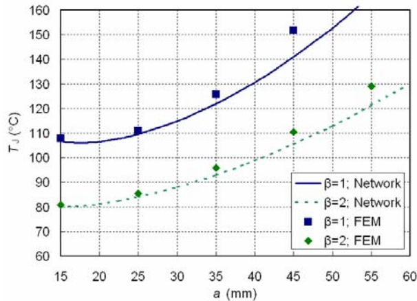
Figure 9. T_j of the LED tube for different a and \beta
