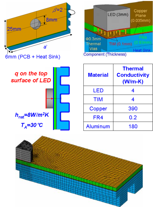
Figure 11. Details of FE Model
