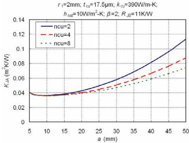
Figure 7. Effect of a on K_{JA} for different t_{fin}
