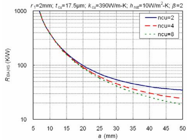
Figure 5. Effect of a on R_{BA,HS} for different t_{fin}
