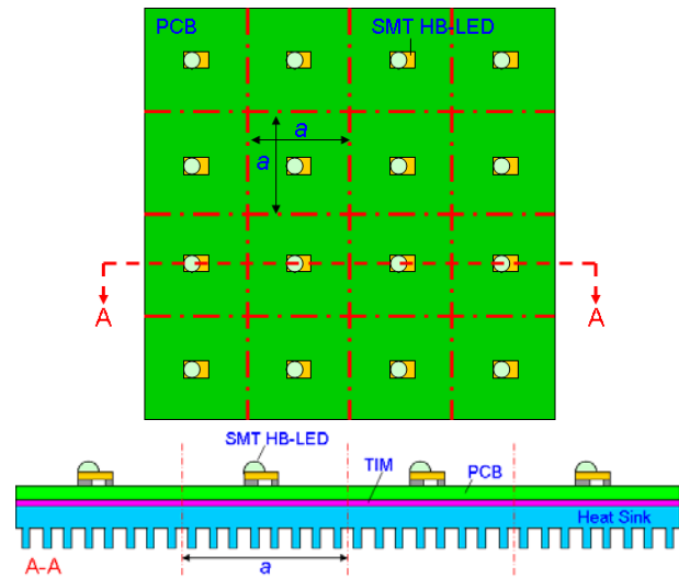
Figure 1. An Array of LEDs with Pitch a
