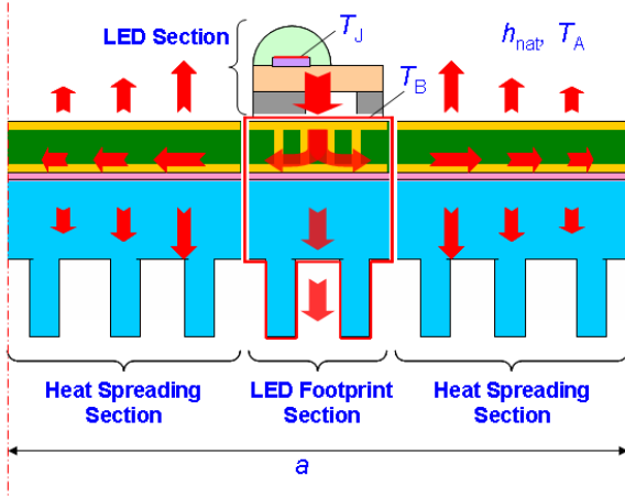
Figure 2. Heat Flow in a Unit Cell
