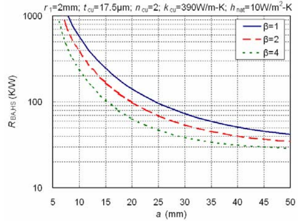
Figure 4. Effect of a on R_{BA,HS} for different \beta
