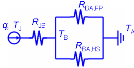
Figure 3. Thermal Network for Thermal Analysis
