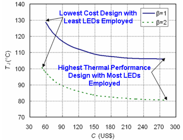
Figure 10. Thermal Performance-Cost Relationship of the LED tube for different \beta
