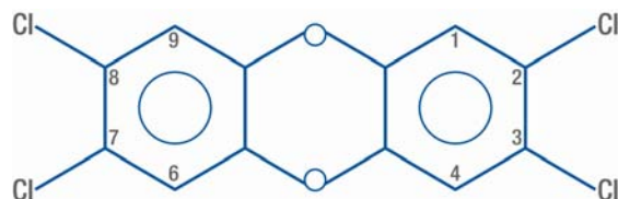
Figure 2: 2,3,7,8 tetrachlorodibenzo-p-dioxin (TCDD)
