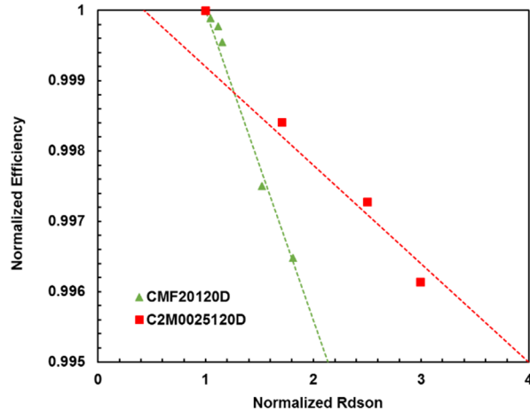
Figure 8 The anode power supply efficiency vs. normalized MOSFET on-state resistance.
