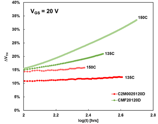
Figure 5 The threshold voltage drift due to 20V gate bias of CREE CMF20120D and C2M0025120D devices.
