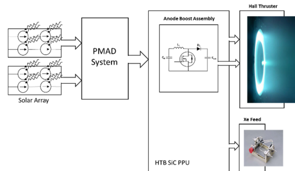
Figure 1 A schematic representation of a solar electric propulsion (SEP) architecture for in-space solar electric propulsion with integrated High Temperature Boost (HTB) Power Processing Unit (PPU). Photonic energy is converted to electricity by the solar array and the resultant energy is regulated and distributed by the Power Management and Distribution (PMAD) system providing an unregulated output power to the PPU. The anode power assembly module is composed of a typical straight boost design utilizing commercially available SiC MOSFETs and diodes for switching.
