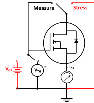
Figure 2 A schematic of High Temperature Gate Bias characterization setup.
