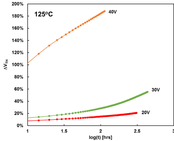
Figure 4 The threshold voltage drift due to 20V, 30V and 40V V_{GS} at 125 °C.
