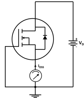
Figure 3 A schematic of High Temperature Reverse Bias characterization setup.
