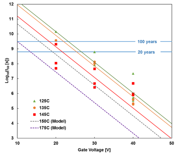
Figure 6 The predicted lifetimes using measured t_{50} and the Eyring model. The lifetime is based on experimental HTGB data measured at 20V, 30V, and 40V V_{GS} .
