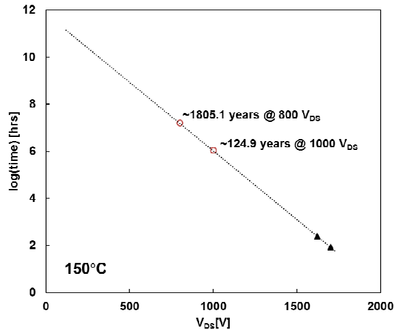
Figure 7 The HTRB voltage accelerated drain-source junction integrity test suggests reliability of over 120 years with 1000V V_{DS} at junction temperature of 150 °C.
