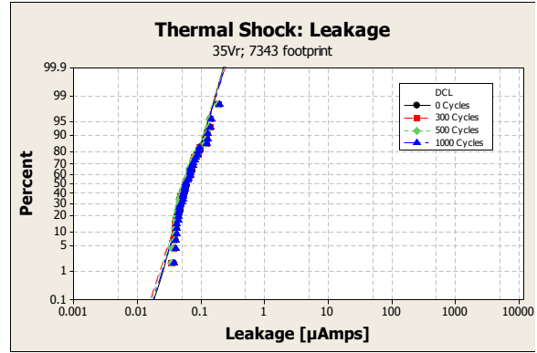
Figures 26, 27, 28. The capacitance, ESR and leakage of 35V rated solid tantalum capacitors are stable through 1,000 cycles of Thermal Shock.
