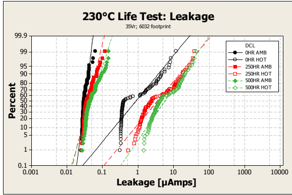
Figures 23, 24, 25. The capacitance, ESR and leakage of 35V rated, 6032 footprint solid tantalum capacitors are stable through 500 hours of life test at 230C.
