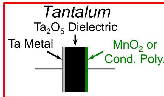
Figure 1. Tantalum, tantalum pentoxide, and a primary cathode material comprise the basic elements of a solid electrolytic tantalum capacitor.
