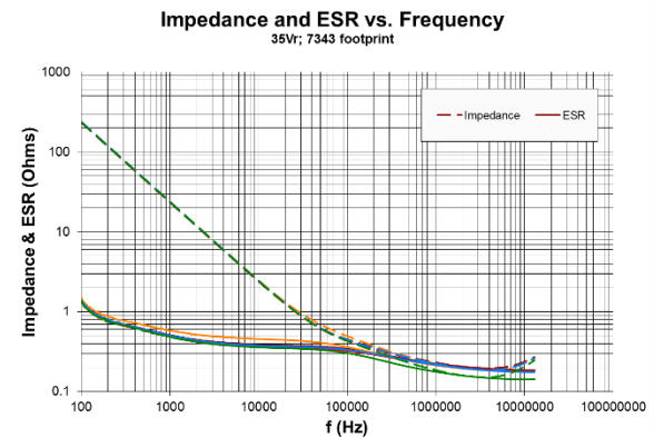
Figures 29, 30. Capacitance vs Frequency and Impedance/ESR vs Frequency of 35V rated solid tantalum capacitors.
