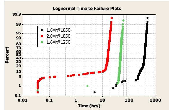
Figure 4. Time to failure curves for solid electrolytic tantalum capacitors under highly accelerated test conditions clearly show that voltage and temperature accelerate the time to ‘wearout’.
