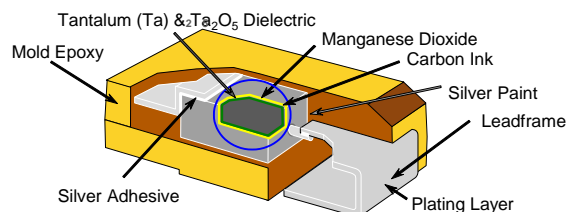
Figure 2. The general construction of a surface mount solid electrolytic capacitor showing
