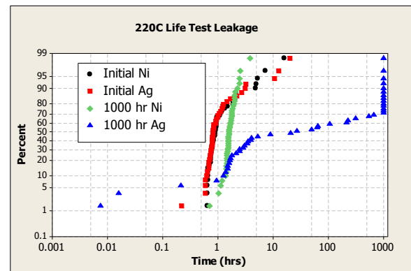
Figure 10. Ta capacitors designed with a silver paint layer are shorts after 1000 hours at 220C, while parts manufactured with an electroplated Ni layer exhibit stable leakage.
