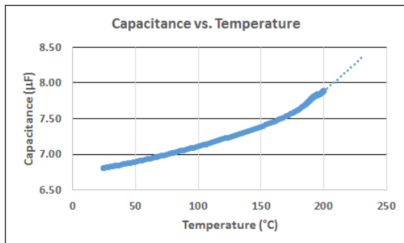
Figure 15. Capacitance of a solid tantalum capacitor rises approximately 22% between 25 and 230C.
