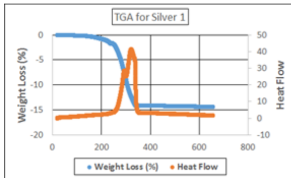
Figures 6 and 7. In contrast to the TGA for MnO 2 , the TGA for a carbon ink and silver paint frequently used for capacitors manufactured for consumer applications exhibit significant degradation in the temperature range of interest to the downhole drilling industry.
