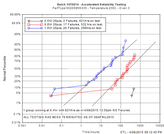
Figures 31. Time to failure testing at 230C for 35V rated solid tantalum capacitor indicates potential for lower derating at application temperature.
