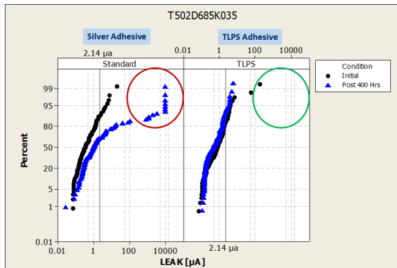
Figure 11. Silver migration from the silver adhesive is eliminated using a transient liquid phase sintering adhesive.
