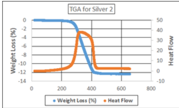
Figures 8 and 9. The TGA of carbon and silver formulations developed for solid electrolytic tantalum capacitors rated for continuous operation at temperatures of 200C and above.
