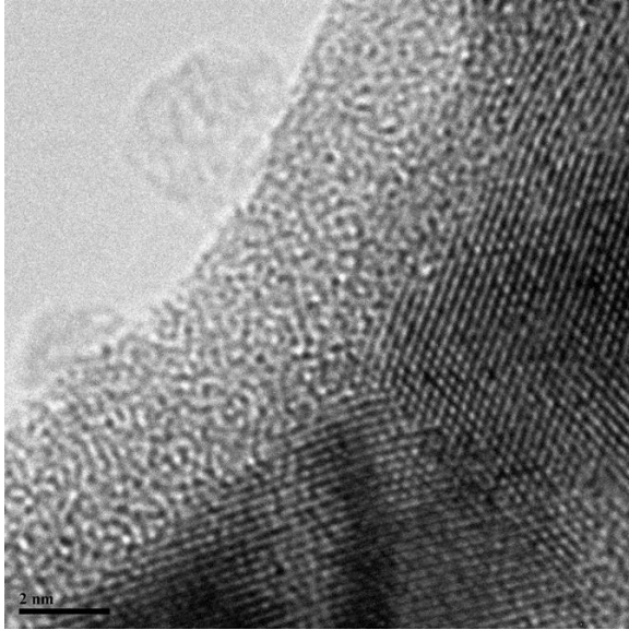
Figure 3. TEM photomicrograph of Ta/Ta 2 O 5 showing the amorphous structure of the Ta 2 O 5 overlying the ordered structure of the tantalum anode (previously published photo).
