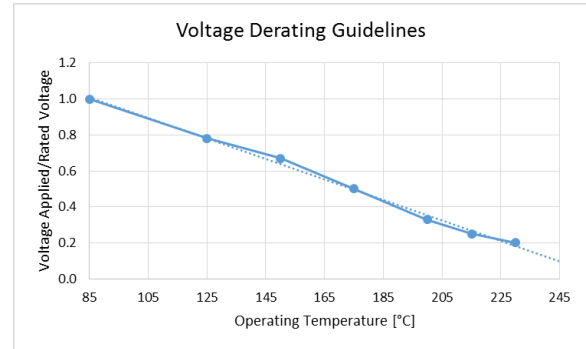
Figure 16. The derating for a tantalum capacitor was calculated by extrapolating traditional derating rules applied at lower temperatures.
