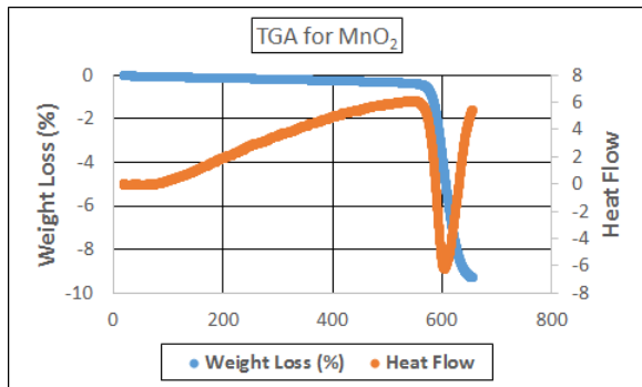
Figure 5. TGA for MnO 2 powder indicates the material is stable up to about 580°C where conversion to non-conductive Mn 2 O 3 occurs.
