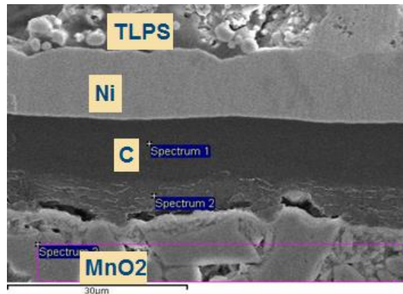
Figure 13. Optimization of the molding compound used to encapsulate the capacitors eliminated the separations between cathode layers resulting in stable ESR during life test.
