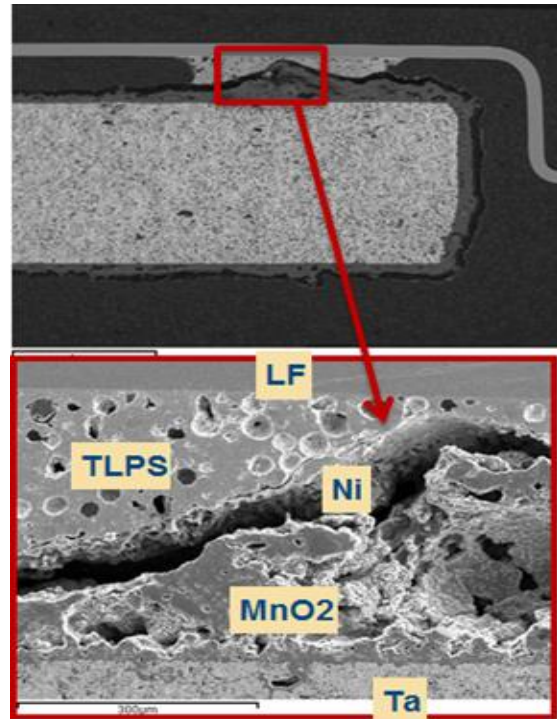
Figure 12. Separation between the cathode layers caused high ESR during high temperature life testing of tantalum capacitors.
