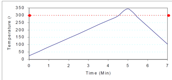
Figure 14. Recommended reflow profile for HMP solder.
