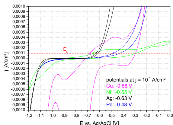
Fig. 7.1: Polarization curve of glyoxylic acid ( c = 0.3 \text{ mol/l} ; pH 13; RT)
