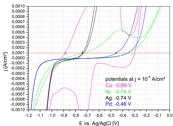
Fig. 7.2: Polarization curve of glyoxylic acid ( c = 0.3 \text{ mol/l} ; pH 13; 40°C)
