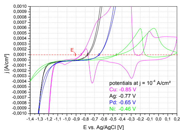
Fig. 6.1: Polarization curve of formaldehyde ( c = 0.3 mol/l; pH 13; 25°C)
